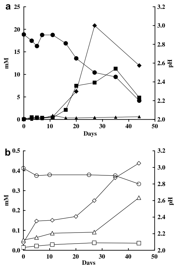
Fig. 2. (a) Change in solution chemistry with time during the oxidation of pyrite by \text{O}_2 in the biological experiments in the presence of A. ferrooxidans . (◆) sulfate; (●) pH; (■) \text{Fe(III)} ; (▲) \text{Fe(II)} . (b) Change in solution chemistry with time during the oxidation of pyrite by \text{O}_2 in the abiotic control experiments without A. ferrooxidans . (◇) Sulfate; (○) pH; (□) \text{Fe(III)} ; (△) \text{Fe(II)} .
